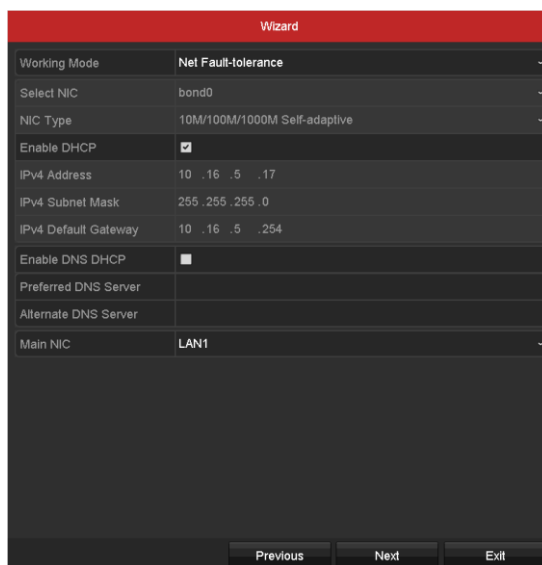
Figure 2-16 General Network Configuration
