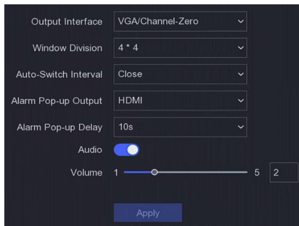
Figure 6-4 Live View-General
