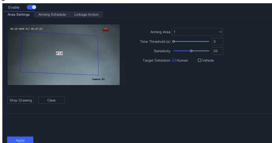
Figure 5-11 Intrusion Detection
