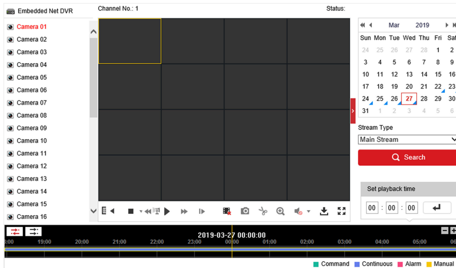
Figure 9-3 Playback
