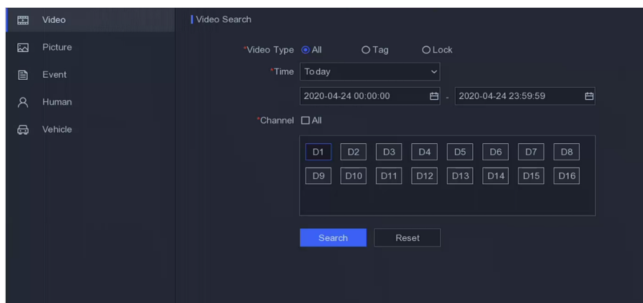
Figure 4-1 Search
