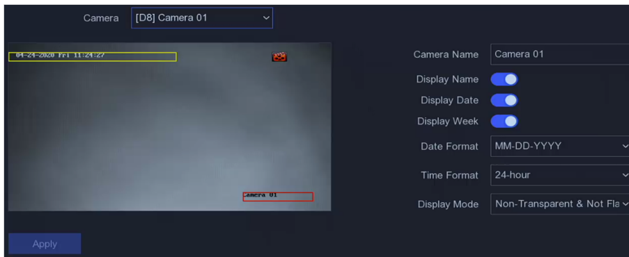
Figure 5-8 OSD
