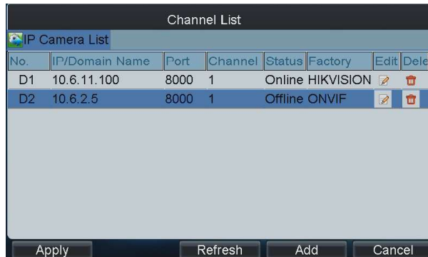
Figure 4.29 IP Camera List
