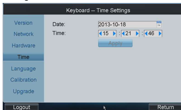
Figure 3.11 Time Settings
