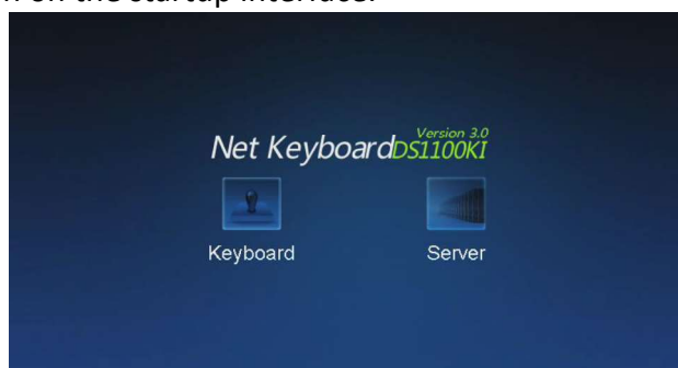
Figure 3.1 Startup Interface
