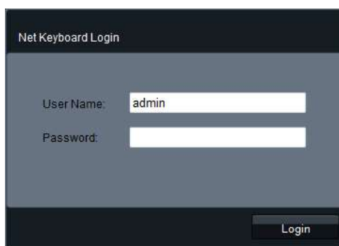
Figure 7.1 User Login
