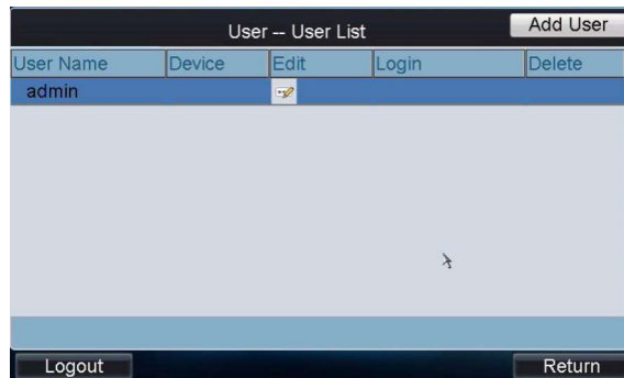
Figure 3.5 User List
