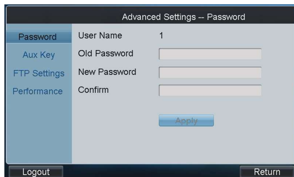
Figure 4.82 Advanced Settings
