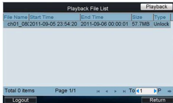
Figure 4.80 Search Result
