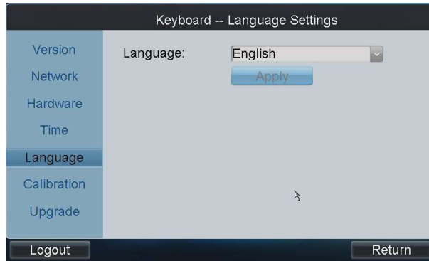
Figure 3.12 Language Settings
