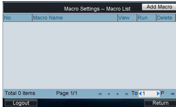
Figure 4.72 Macro Settings
