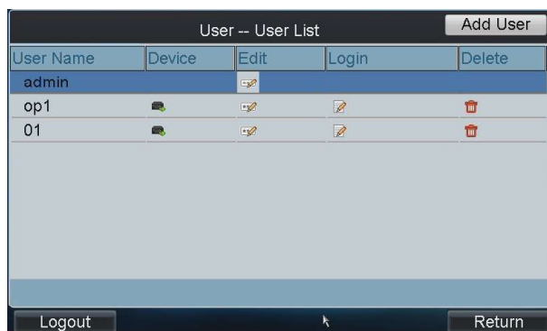
Figure 4.2 Operator Login (2)
