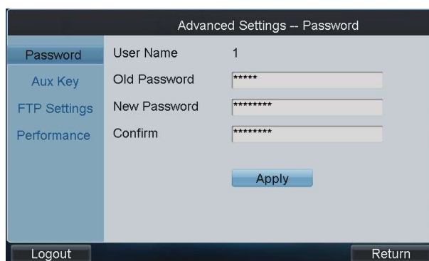
Figure 4.83 Modify Password
