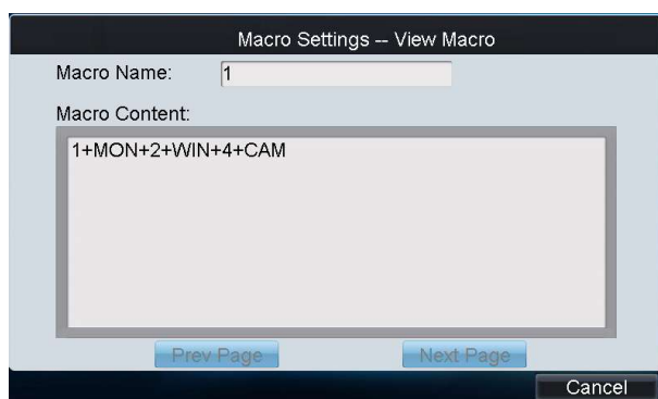
Figure 4.75 View Macro
