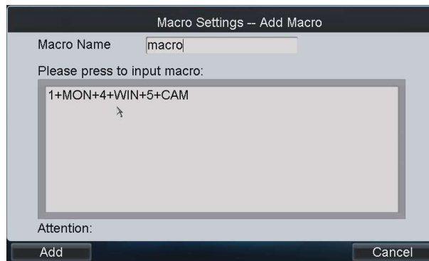
Figure 4.73 Add Macro
