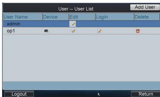
Figure 3.25 User Management
