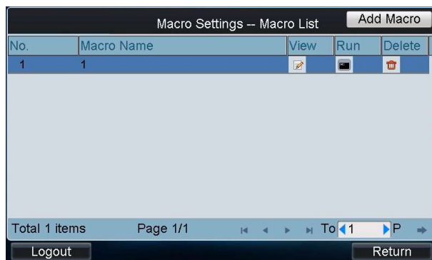
Figure 4.74 Macro List
