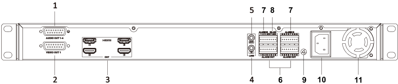
Figure 1-8 DS-6904UDI (C) V3.0.0 Rear Panel
