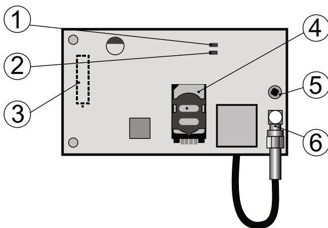
Fig. 1: JA-190Y sender
